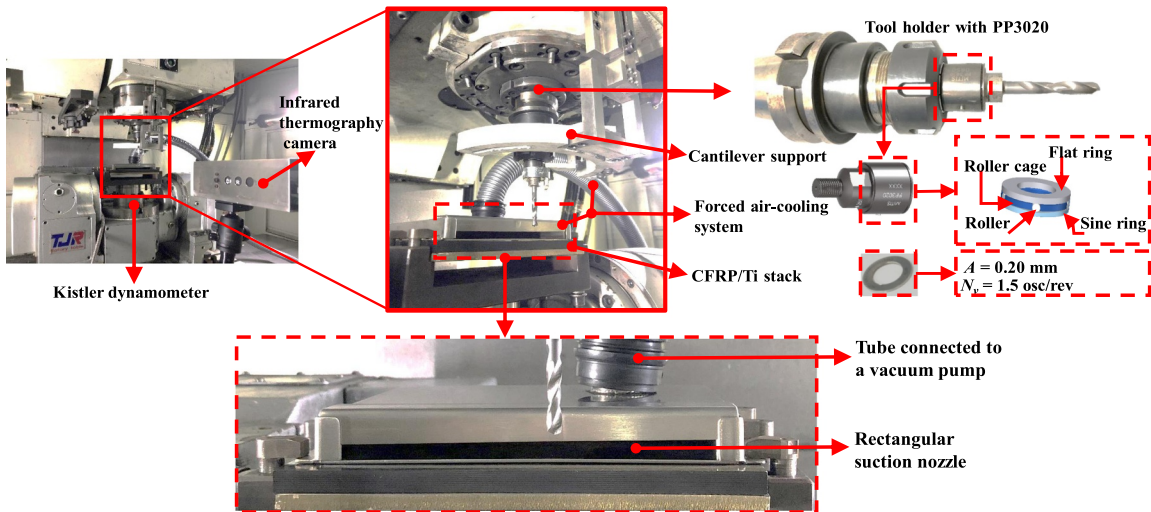
Fig. 2. Photographs showing the experimental setup. Right is the tool holder for the LFVAD and the components of the source of axial oscillations ( A = 0.20 mm and N_v = 1.5 osc/rev) and below is the designed forced air-cooling system.
