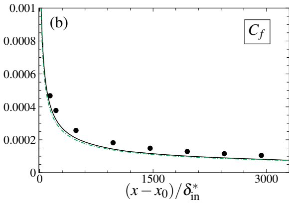
Figure 3: Streamwise evolution of skin friction coefficient C_f . (a) Entire domain and (b) zoom in the laminar region, along with the laminar correlation ( -\cdot-\cdot- ) and the locally self-similar solution (symbols).
