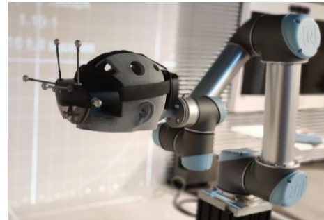
Figure 1: Picture of the 3D printed head installed on the UR5 with a HoloLens 2 mounted on it.
