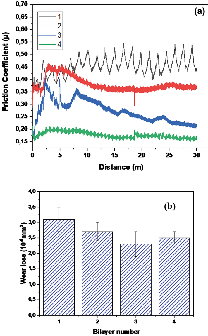
Fig. 3. Friction coefficient of CrN/CrAlN multilayer films in seawater environment, (b) volume loss of CrN/CrAlN multilayer coatings
