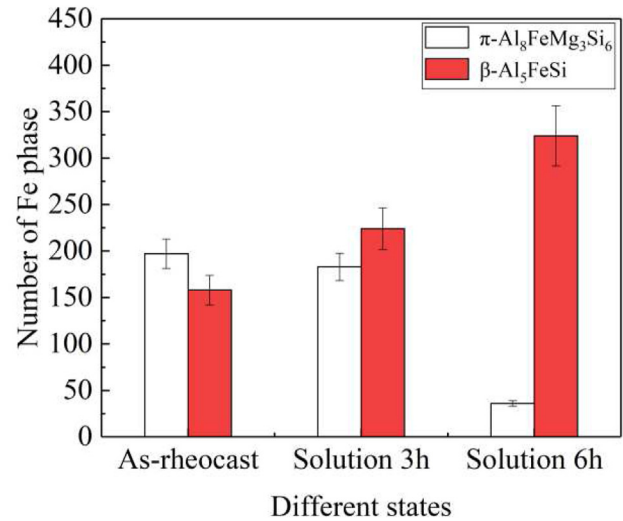
Fig. 6 – Number of Fe-rich intermetallic phases in the alloy for various solution times.
