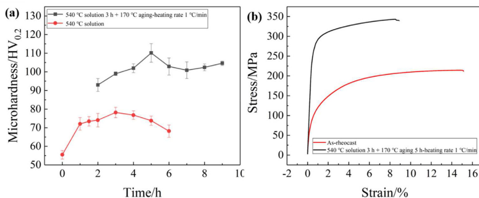
Fig. 9 – Microhardness evolution as a function of solution time and ageing time.
