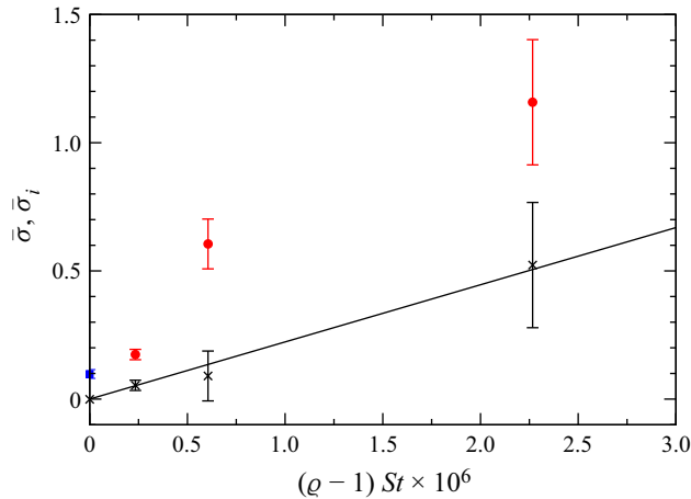
Figure 25. Mean rates of attraction to the period-one limit cycle for inertial particles with \varrho > 1 as functions of (\varrho - 1)St . Shown are the total attraction rates \bar{\sigma} (red dots, blue square) measured and the inertial attraction rate \sigma_i (black crosses) after eliminating the wall effect. Three particles with different radii a \in [0.0069, 0.0120, 0.0130] and corresponding densities \varrho \in [1.022, 1.019, 1.061] were tested. The solid line represents the linear regression \bar{\sigma}_i = c(\varrho - 1)St with c = 2.23 \times 10^5 . The blue square shows \bar{\sigma} for a particle with a = 0.0064 , \varrho = 0.0001 .
