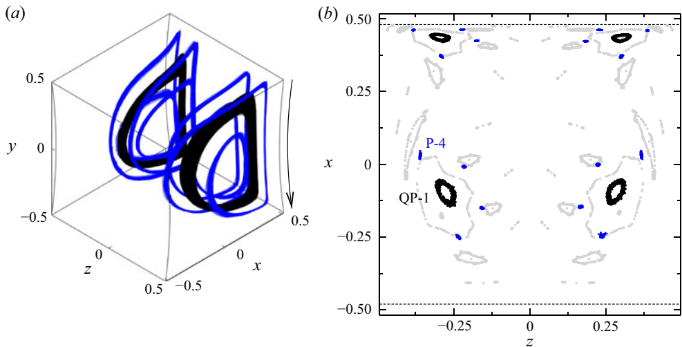
Figure 26. Thirty-seven trajectories for a = 0.0111 ( a_p = 0.45 mm) and \varrho = 0.940 recorded during t \in [1000, 1180] s. (a) Three-dimensional view of the toroidal period-one attractors QP-1 (black) and the stable period-four limit cycles P-4 (blue). (b) Poincaré sections on the plane y = 0 (black, blue) of the particle trajectories shown in (a). Poincaré sections of numerically computed streamlines of characteristic KAM tori are shown as light grey dots.
