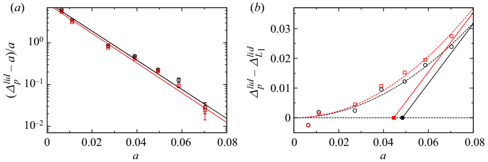
Figure 28. (a) Normalized minimum gap (\Delta_p^{\text{lid}} - a)/a between the surface of the particle and the moving wall for Re = 100 (black, circles) and Re = 200 (red, squares) on a logarithmic scale. The solid lines are weighted exponential fits according to 9.6e^{-80.5a} (black curve, Re = 100 ) and 8.7e^{-82a} (red curve, Re = 200 ). (b) Distance \Delta_p^{\text{lid}} of the limit cycle P-1 from the moving wall relative to the distance \Delta_{L_1}^{\text{lid}} of the closed streamline L_1 from the moving wall as a function of the particle radius a for Re = 100 (black, circles) and Re = 200 (red, squares). The dashed lines are quadratic fits of the form ca^2 with c = 103 ( Re = 100 ) and c = 129 ( Re = 200 ). The solid lines indicate the prediction of the model of Hofmann & Kuhlmann (2011).
