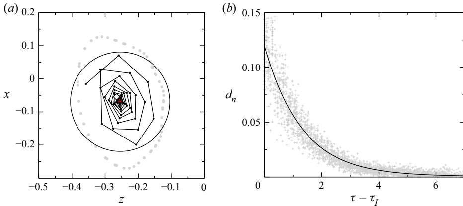
Figure 9. (a) Poincaré section on y = 0 of a trajectory of a single particle (black dots and lines) with a = 0.0272 and \varrho = 1.0001 . The final phase from \tau = 6.4335 onwards is shown by red dots. Grey dots indicate the largest contiguous KAM torus; the white diamond marks the closed streamline; and the circle defines the threshold distance d^* for Poincaré points to be included in the fit (5.3). (b) The distance function d_n for 40 realisations (grey plus signs). A fit (solid black line) of the data according to (5.3) yields the attraction rate \bar{\sigma} = 0.766 \pm 0.07 .
