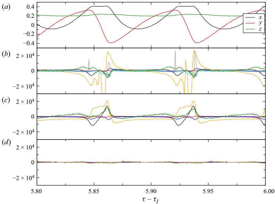
Figure 14. (a) Trajectory ( x, y, z ) of the particle with a = 0.0704 and \varrho = 1.0001 for Re = 100 moving on its attractor. (b–d) Different components of the acceleration in the x , y and z directions, respectively. For an explanation of the colour code, see the text.
