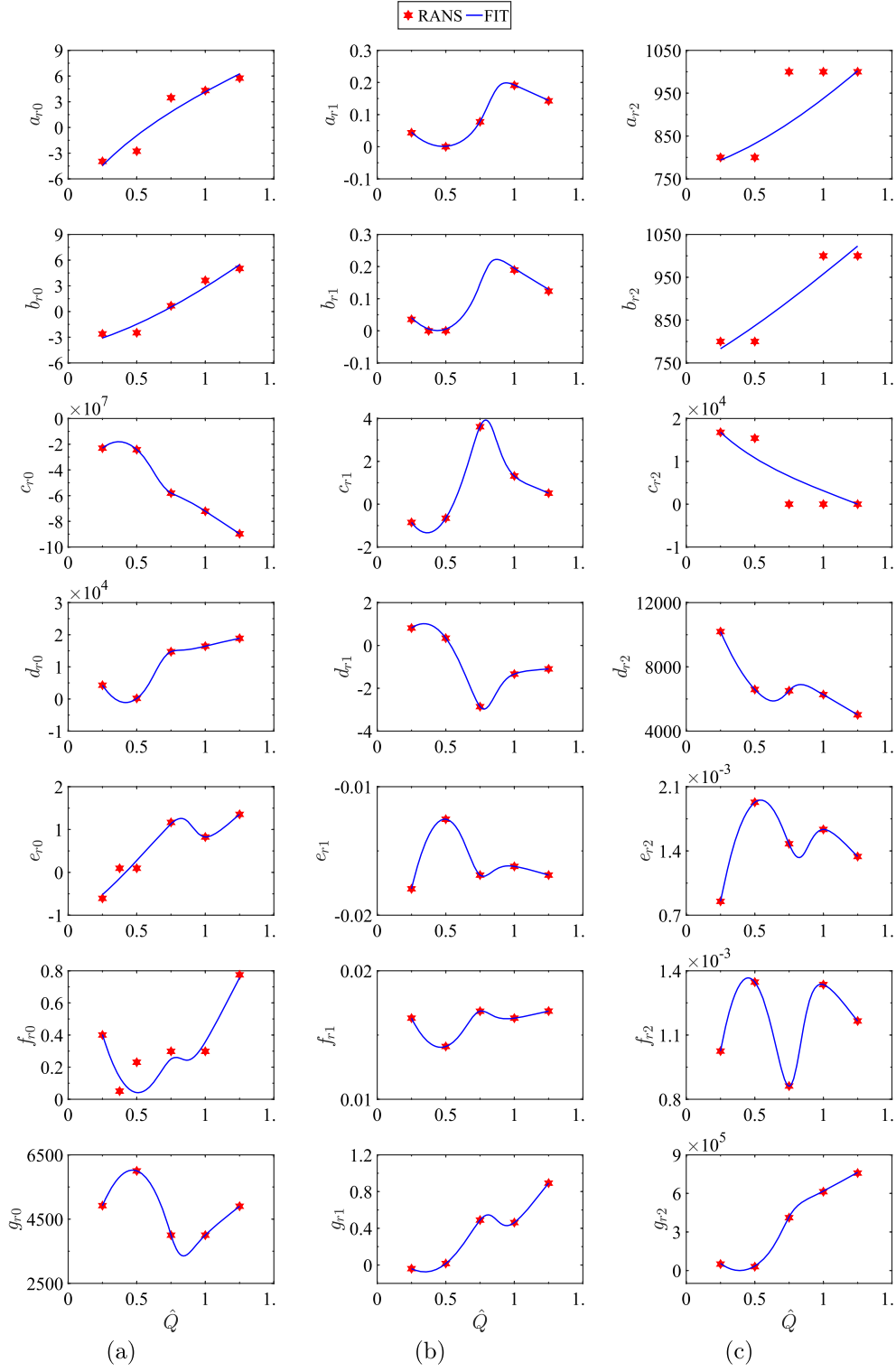
Fig. 12. Secondary fitting for the coefficients \dagger_{ri} of U_r with the rotational speed \omega_{\text{imp}} = 125 rad/s and diffuser radius ratio \Gamma = 1.50 of the positive-leakage case.
