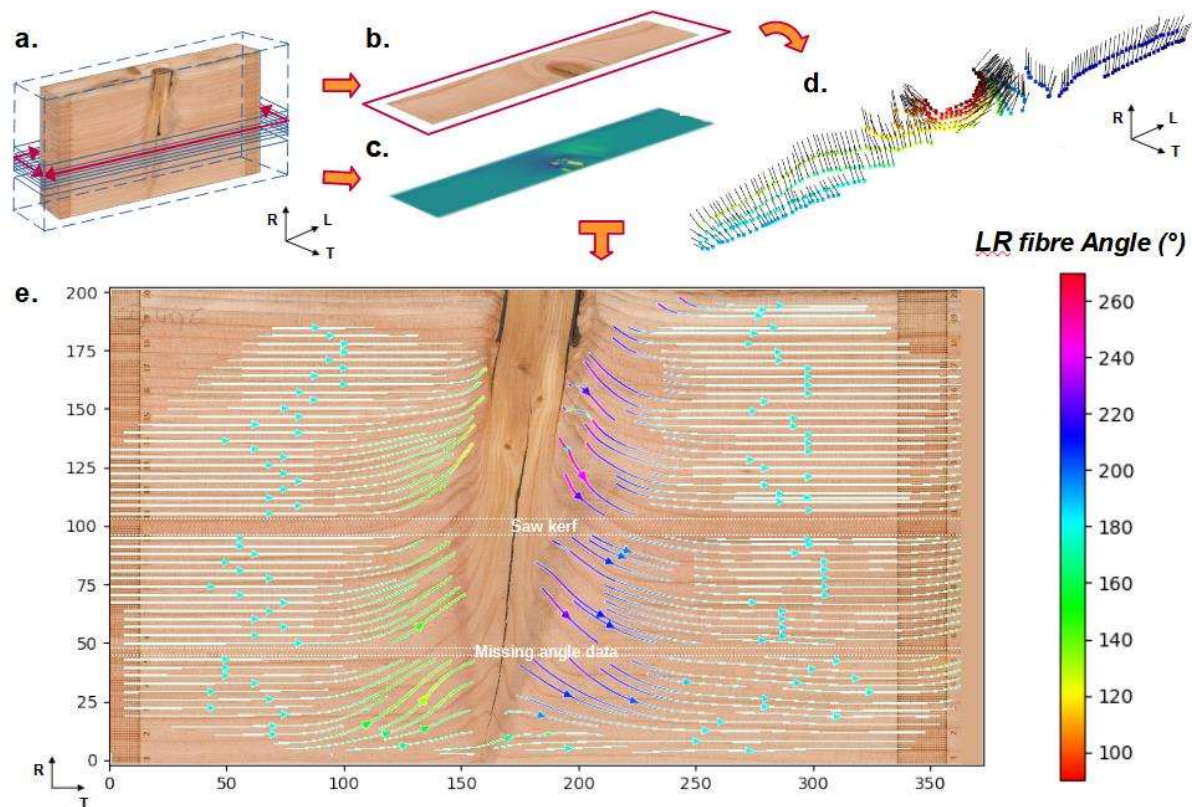
Figure 1. shows a. the original sample, which has been cut into two halves in order to fasten the following successive 2-mm planing with an industrial planing machine – b. colour scanning – c. LT in-plane fibre angles measurement with a laser point machine. After detecting growth-layer on the colour scans, d. a point cloud is made of the boundary growth-ring surfaces , and normals of these surfaces estimated. e. Streamplot showing the resulting LR in-plane fibre orientation overlaid on the sample side colour scan .
