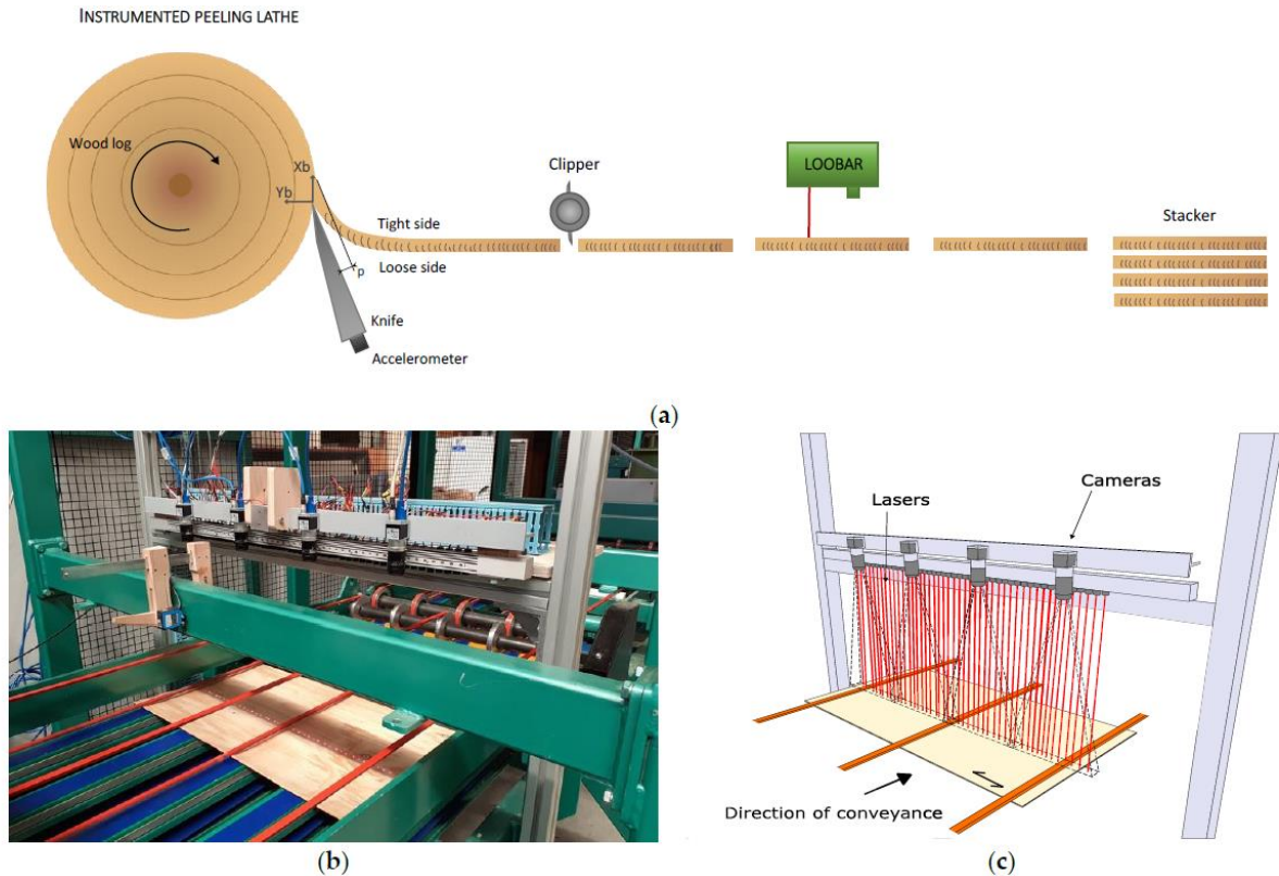
Figure 1: The LOOBAR, a veneer fiber orientation-measurement: (a) schematic representation of LaBoMaP's instrumented rotary peeling line, (b) picture, and (c) scheme of the LOOBAR.
