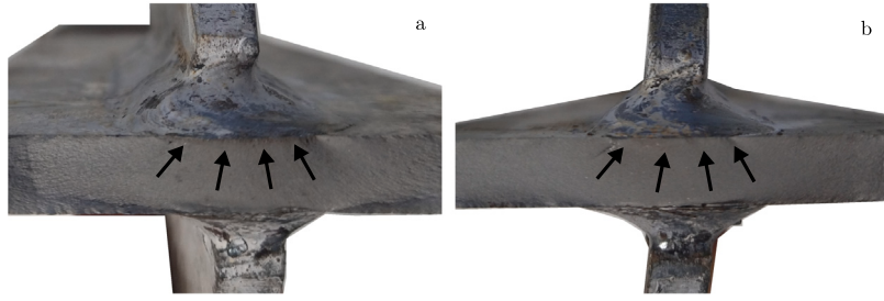
Fig. 14. Fracture surface of (a) an as-welded and (b) a proof-loaded structure, cyclically tested with a load ratio of R = 0.1 . Multiple crack initiation sites can be observed at the weld toe surface.
