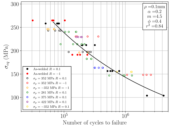
Fig. 16. Numerically determined "master S-N curve" obtained for stiffener structures for different load ratios for as-welded and proof-loaded specimens. A heterogeneous description is adopted for the FEM simulations. Both the strain hardening effect and the role of the maximum hydrostatic pressure are considered for the application of the fatigue criterion.
