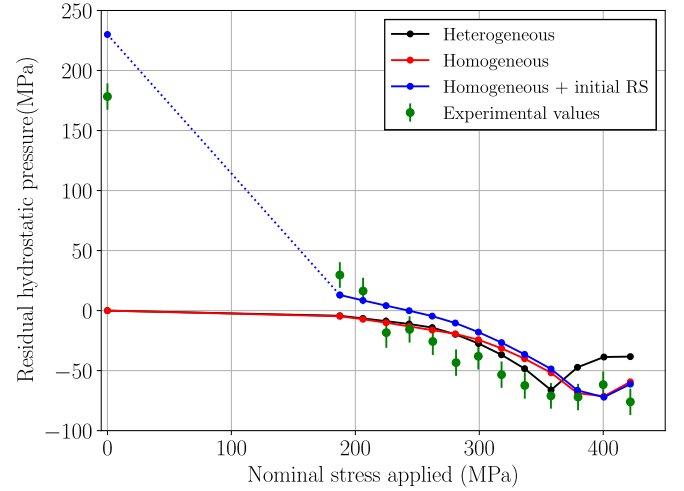
Fig. 13. Comparison between the residual hydrostatic pressure determined experimentally and via numerical simulations after proof load. The dotted line indicates a region where interpolation between the corresponding data points is uncertain.
