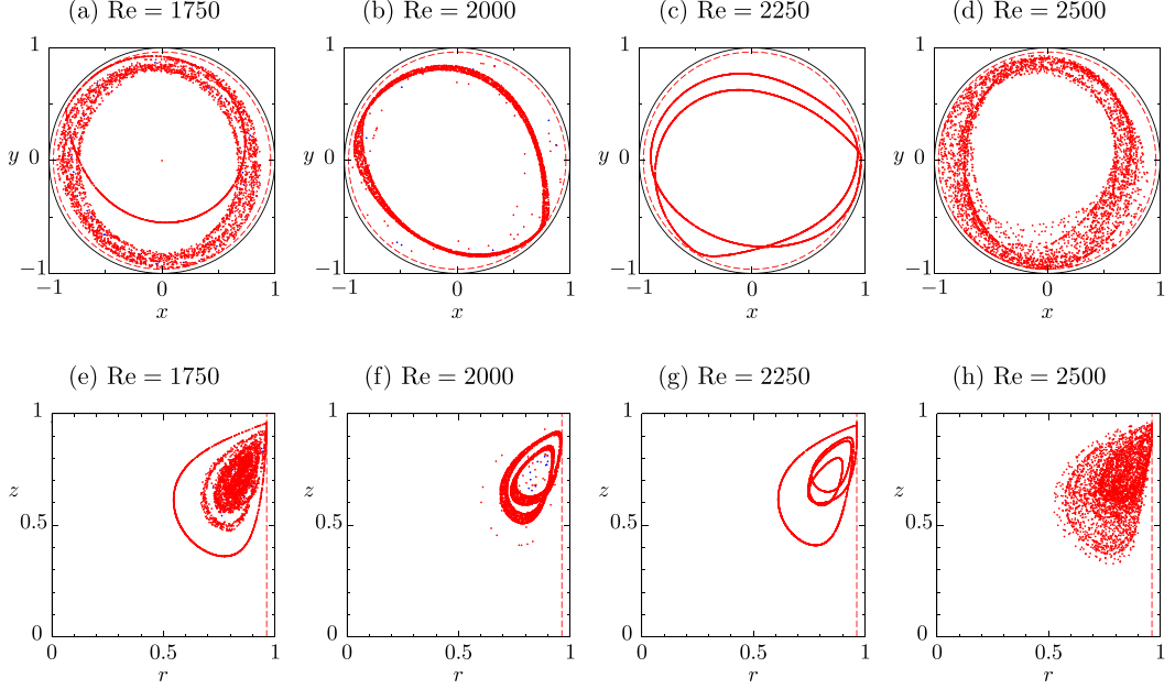
FIG. 20. Particle accumulation structures for q = 1 , \Delta = 0.037 and different values of Re as indicated. Shown are axial (top) and azimuthal (bottom) projections of the particle configuration at t = 5 . Lines, symbols, and colors as in Fig. 16.
