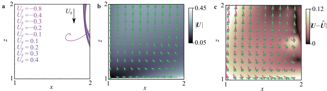
Figure 7 Set of particle trajectories selected for reconstructing the neutrally-buoyant particulate flow a , particle velocity field for U_g = 0 b , and reconstructed flow absolute error c . The green arrows show the target flow and the pink arrows denote the reconstructed particle flow.
