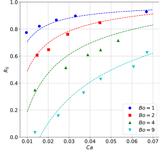
FIG. 10. The split ratio, R_S vs Ca . For Bo = 1, 4 , and 9 , r_0 = 10^{-3} , 2 \times 10^{-3} , and 3 \times 10^{-3} m, respectively, at a fixed \sigma = 10^{-2} N/m. For Bo = 2 , r_0 = 2 \times 10^{-3} m and \sigma = 2 \times 10^{-2} Pa m. Ca is calculated from the resultant plug speed, \bar{U} . Dashed lines are computed using Eq. (C1).
