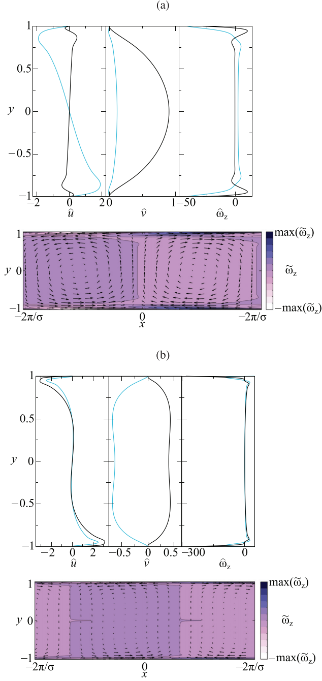
FIG. 6. Top panels: real (black) and imaginary (light blue) parts of the neutral eigenmode in terms of \hat{u} (left), \hat{v} (center), and \hat{\omega}_z (right). Bottom panel: the most dangerous perturbation depicted in terms of vorticity and velocity field (arrows). Critical conditions for the power-law basic state u_0 = 1 - y^2 for \alpha = 2 (a) and \alpha = 4 (b).
