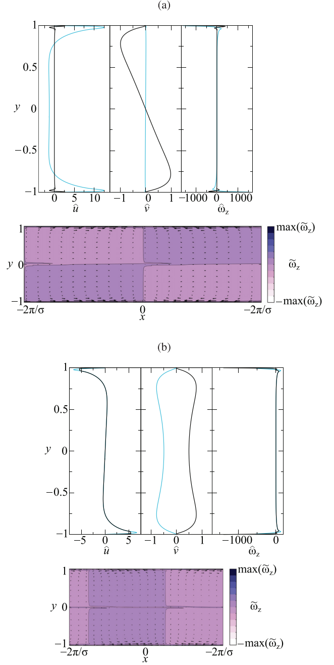
FIG. 7. Top panels: real (black) and imaginary (light blue) parts of the neutral eigenmode in terms of \hat{u} (left), \hat{v} (center), and \hat{\omega}_z (right). Bottom panel: the most dangerous perturbation depicted in terms of vorticity and velocity field (arrows). Neutral conditions (\text{Re}, \sigma) = (366\,400, 1.00) for the power-law profile for \alpha = 8 (a) and critical conditions for \alpha = 8 (b).
