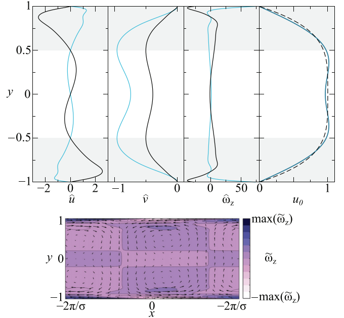
FIG. 9. Top panels: real (black) and imaginary (light blue) parts of the neutral eigenmode in terms of \tilde{u} (left), \tilde{v} (center-left) and \tilde{\omega}_z (center-right), and basic state u_0 (light blue, right) for the generalized Kolmogorov flow for \alpha=4 and K=2 . The dashed line in the top-right panel shows the power-law profile for \alpha=4 and the gray stripes highlight the region where the eigenmode admits the highest velocity and velocity gradients. Bottom panel: the most dangerous perturbation depicted in terms of vorticity and velocity field (arrows). Critical conditions for the generalized Kolmogorov flow for K=2 and \alpha=4 are considered.
