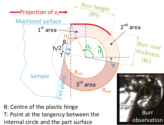
Fig. 10 Geometrical model of burr accumulation before contact with the workpiece. View from a plane normal to the part exit edge
