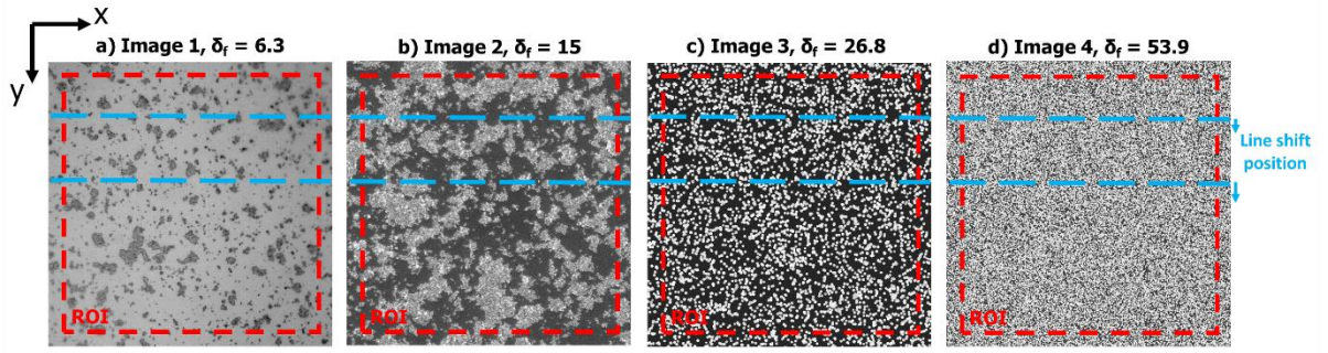
Figure 16. SEM image and virtual image used to evaluate the impact of the speckle on the statistical parameters.
