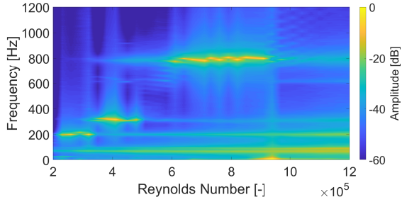
FIGURE 4 – Vibration response spectrum as a function of the Reynolds number for an angle of attack of 5^\circ
