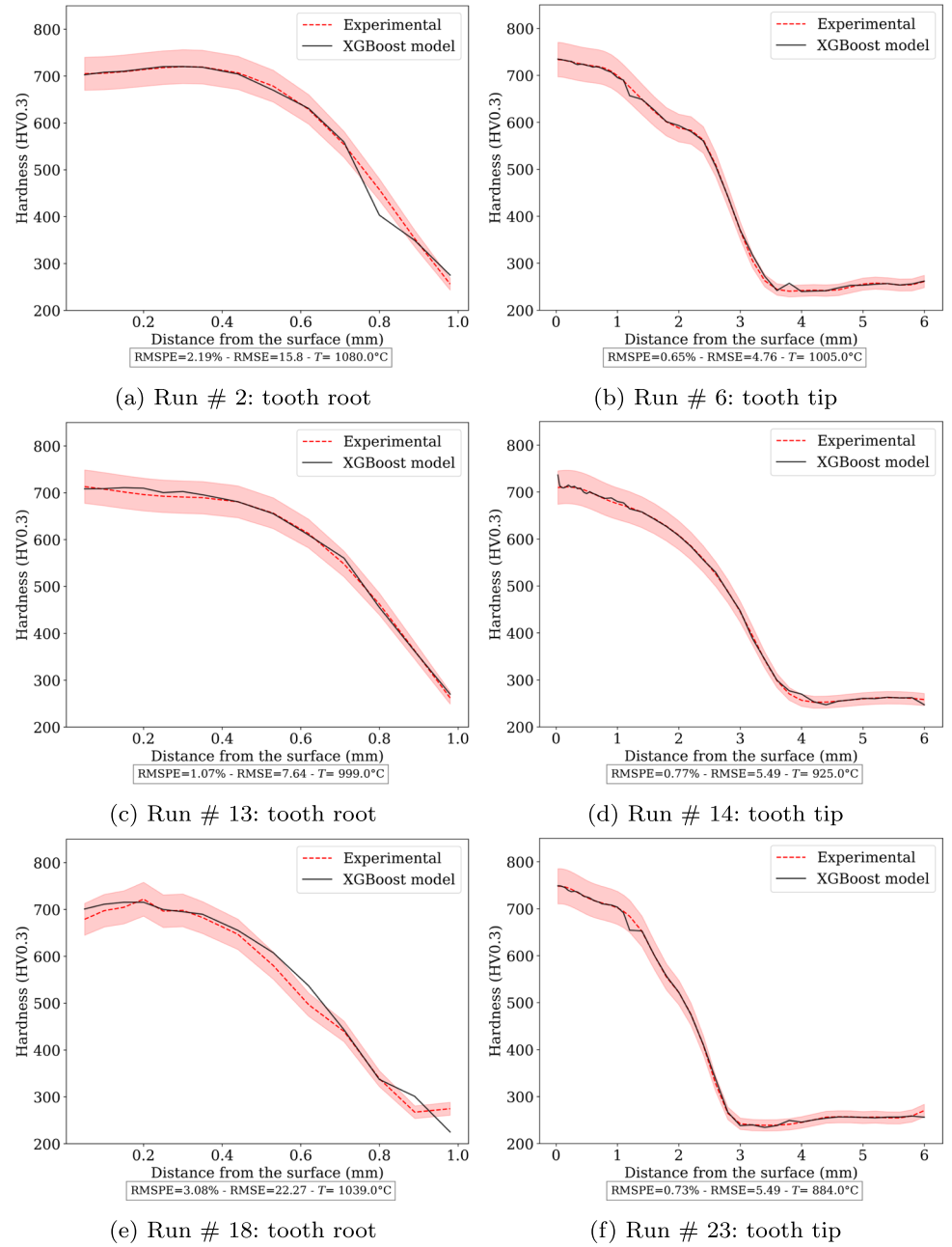
Fig. 10 Comparison of the XGBoost model with the experimental hardness for the gear treated under double frequency - Case 2. T is the measured surface temperature
