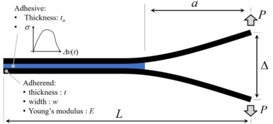
Fig. 1 Schematic representation of a DCB test
