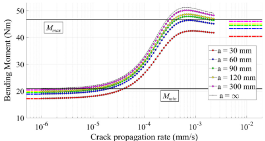
Fig. 13 Crack propagation rate (logarithmic scale) as a function of applied moment for different initial crack lengths for viscoelastic interface behaviour
