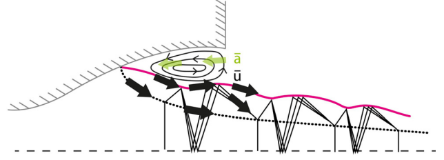
FIG. 23. Sketch of the mechanism linked to the high-frequency modes. The hydrodynamic mode at St = 0.3 is related to a perturbation conveyed with a velocity \bar{u} in the external supersonic shear layer. The screech-like mode is related to the perturbation radiating at the speed of sound \bar{a} . Both modes are the expression of a Kelvin-Helmholtz instability at \overline{St} \approx 0.65 . The large-scale flow maintaining the feedback loop is the recirculation bubble at the nozzle lip.
