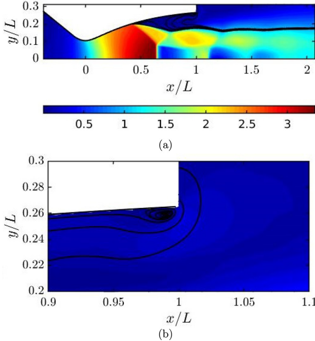
FIG. 22. Contours of the mean Mach number \bar{M} at NPR=9. Streamlines are denoted with a solid black line. (b) is a zoom of the recirculation region near the nozzle lip.
