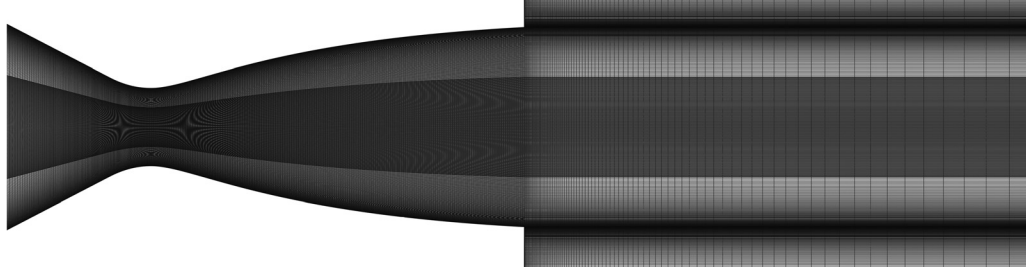
FIG. 4. Computational grid used in the calculation. Longitudinal cut plane.
