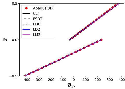
(a) a/h = 100
