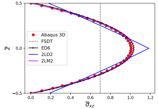
(c) a/h = 5
