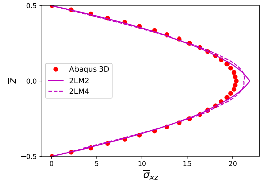
(a) a/h = 100
