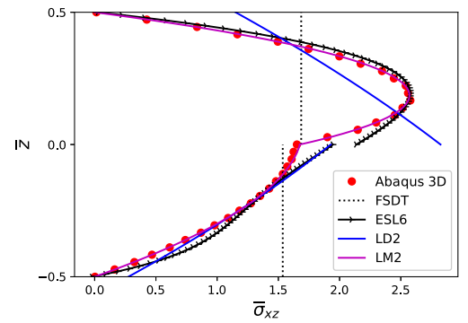
(b) a/h = 10
