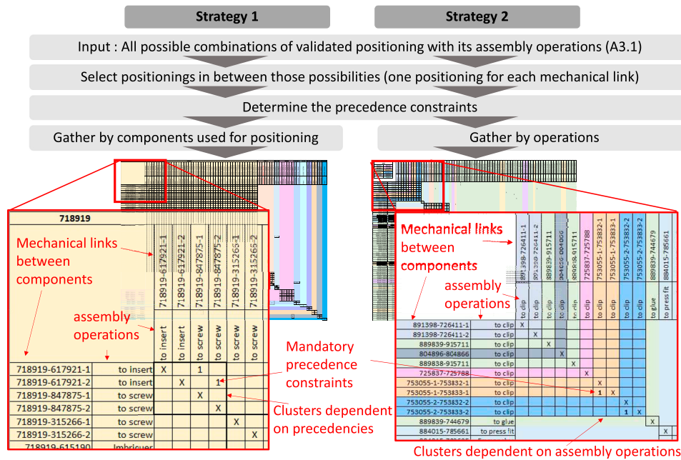
Figure 12. Strategies for the final determination of positioning in the assembly system.
