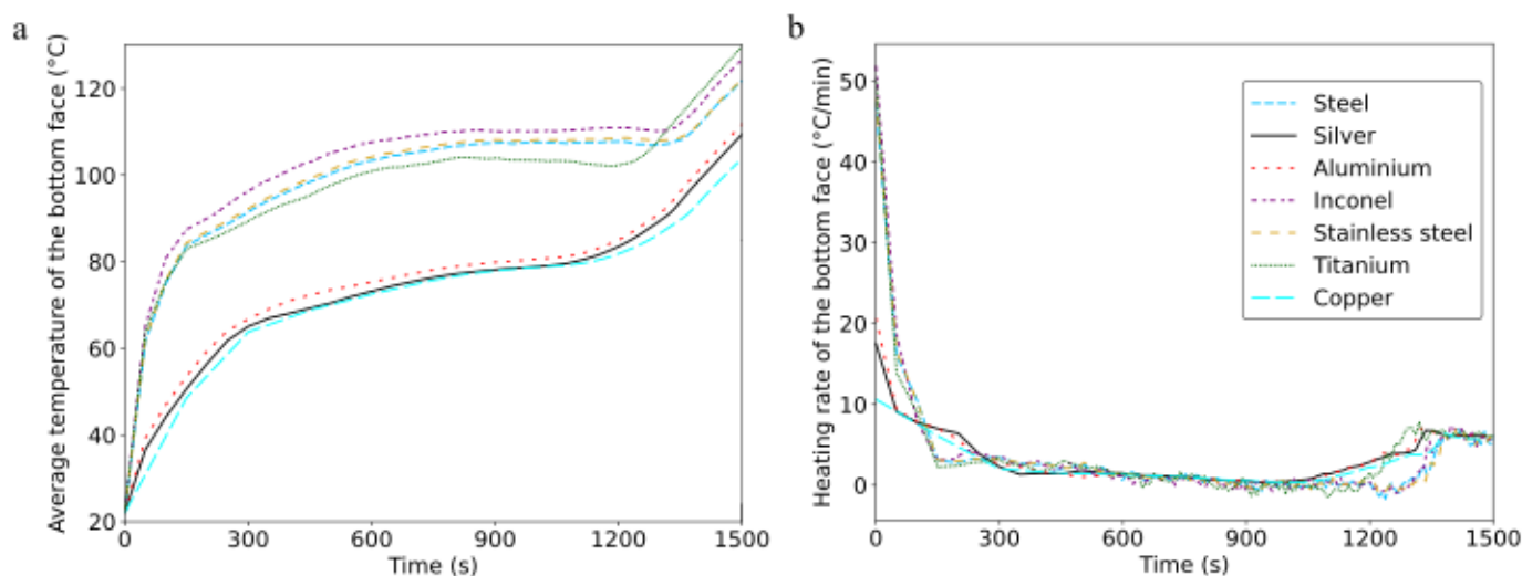
Fig. 6. a) Average temperature of the bottom face of the porous architected structure against time. b) Heating rate of the average temperature of the bottom face of the porous architected structure against time.
