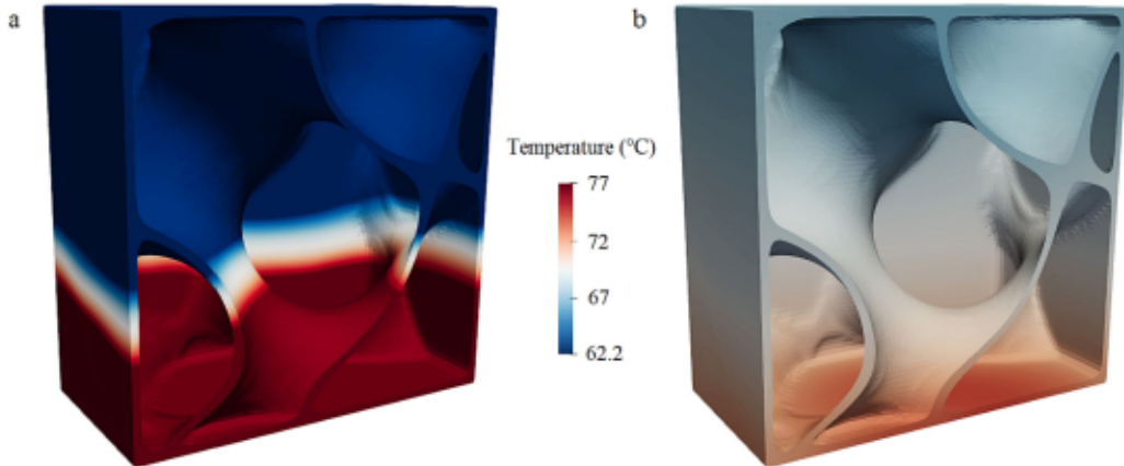
Fig. 4. Temperature of the structure impregnated with PCM after 10 min of heating using a) steel, b) copper.
