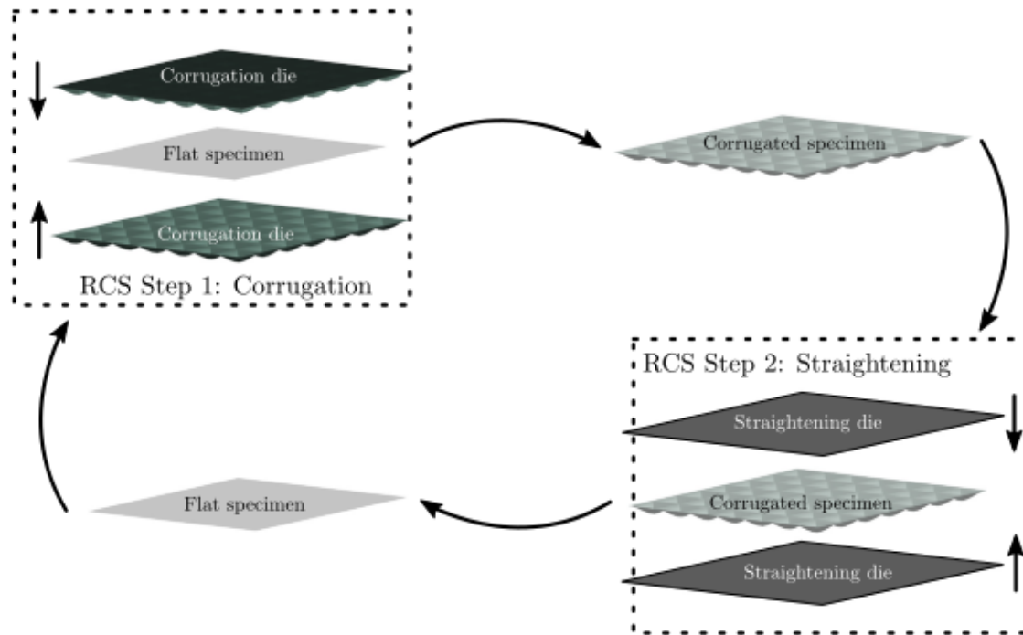
Fig. 2. Description of processing by repetitive corrugation and straightening.
