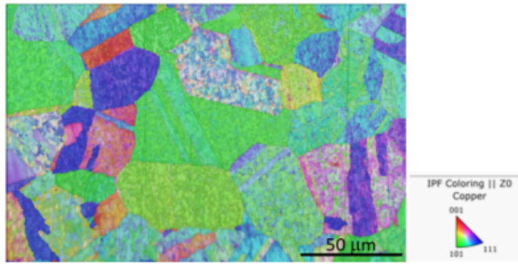
Fig. 1. Characteristic microstructure of Cu samples prior to RCS process. (For interpretation of the references to color in this figure legend, the reader is referred to the web version of this article.)
