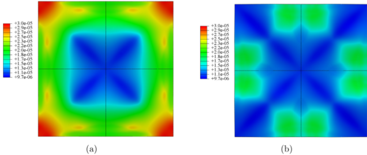
Fig. 13. Distribution of average cell size d (in m) after (a) Pass 1 and (b) Pass 2. The value before processing is d_0 = 32.3 \text{ }\mu\text{m} .
