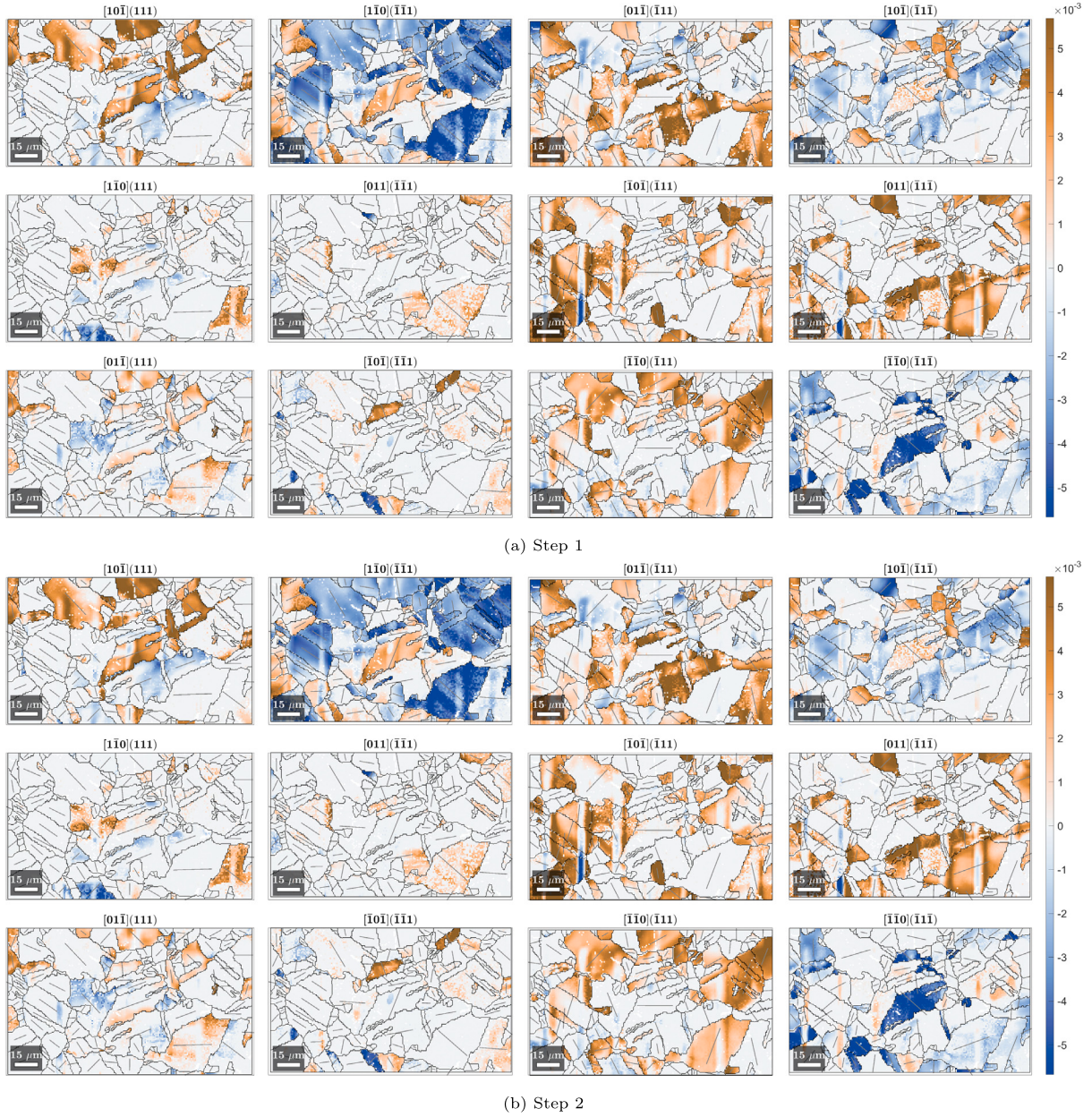
Fig. 17. Slip activities, computed from DIC measurements made with \varphi = 9.6 \mu\text{m} .
