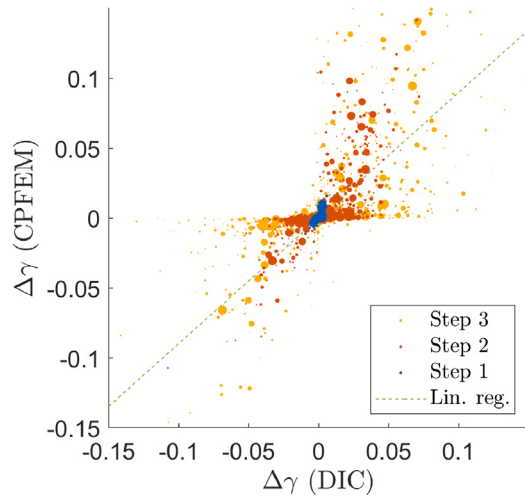
Fig. 23. Grain-wise mean activities computed from CPFEM vs. mean activities estimated from DIC (through the Energy method with \varphi = 1.3 \mu\text{m} ). The dot sizes are proportional to the grain areas.
