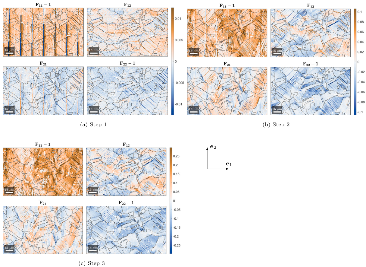
Fig. 2. Components of the gradient ( \mathbf{F} ) given by HR-DIC with \varphi = 1.3 \mu\text{m} at each step (blue dots in Fig. 1(a)). Grain boundaries are drawn in black.
