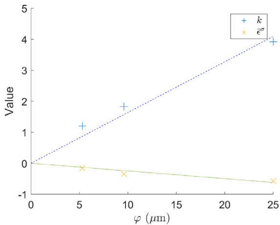
Fig. 19. Slopes of the envelope of \epsilon^E(k) and mean values of \epsilon^\sigma as functions of the window size. The dashed and the dash-dotted line show the linear regressions (33) on k and \epsilon^\sigma , respectively.
