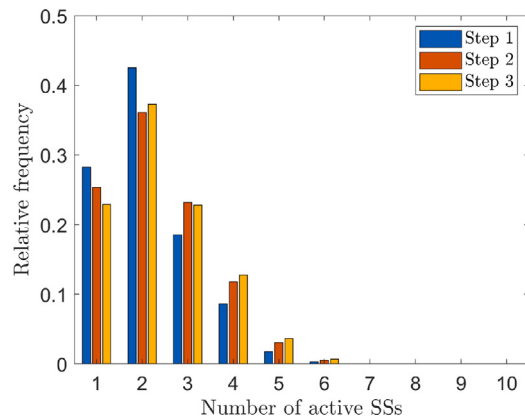
Fig. 24. Histograms of the numbers of active slip systems ( \rho ) for each step, computed from CPFEM.
