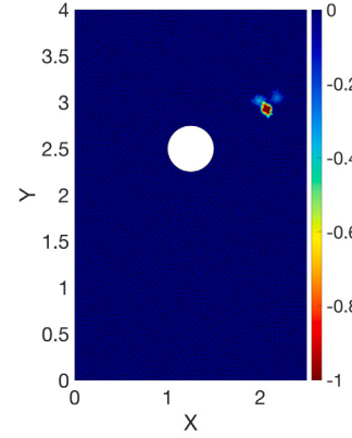
(b) Coefficients a_i in the entire structure representing the identification of the damage.
