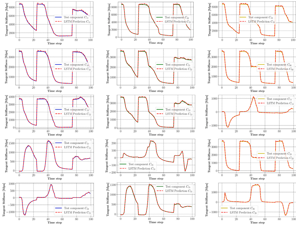
Fig. 15. LSTM predicted macroscopic tangent matrix components in comparison to the RVE FE simulation for an example of test data (Only the symmetric part and the significant components are showed).
