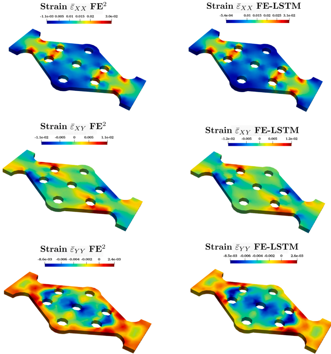
Fig. 18. Comparison between the macroscopic strain fields \bar{\epsilon} obtained by \text{FE}^2 and by FE-LSTM of an architected specimen with holes under tensile loading.
