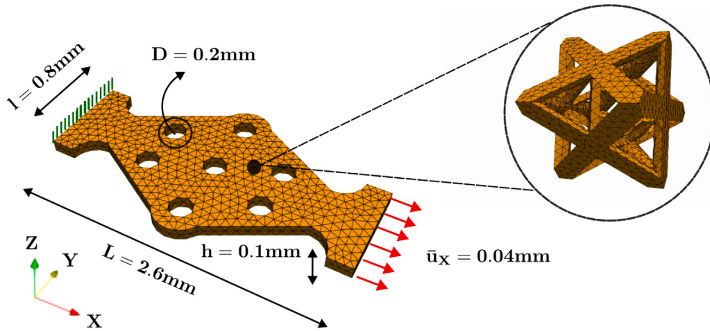
Fig. 16. Geometry, mesh and boundary conditions of an architected specimen with holes under tensile loading.
