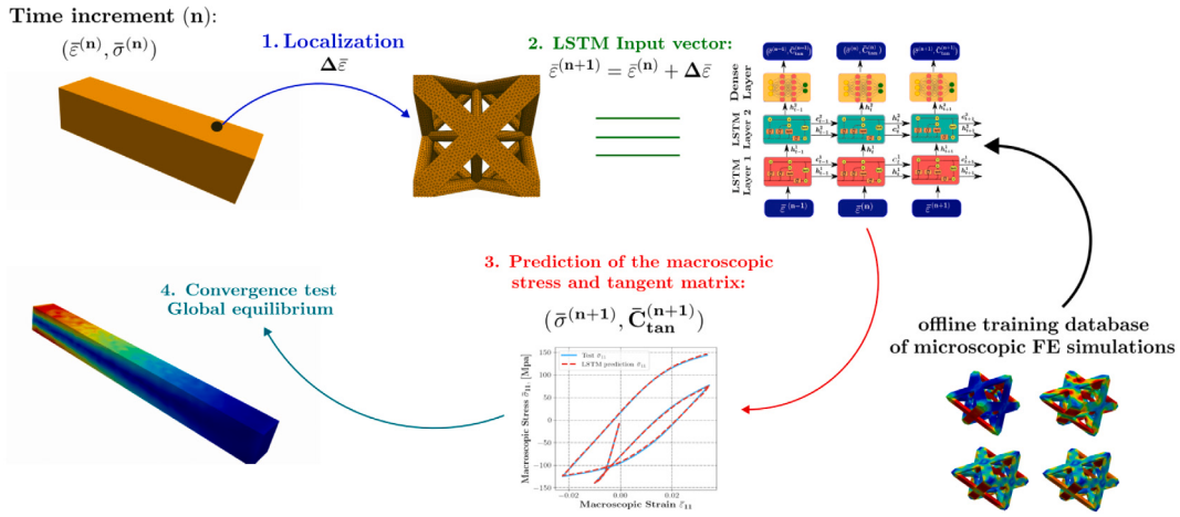
Fig. 6. FE-LSTM general workflow to compute the effective mechanical response of non-linear heterogeneous structures.
