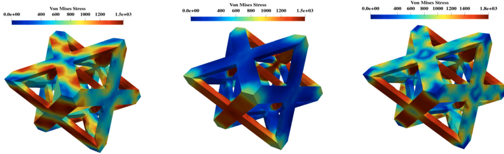
Fig. 10. Examples of simulated octet-truss using FE analysis, the corresponding homogenized fields are used as training data.
