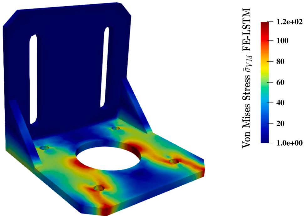
Fig. 22. Macroscopic Von Mises stress \bar{\sigma}_{VM} distribution.
