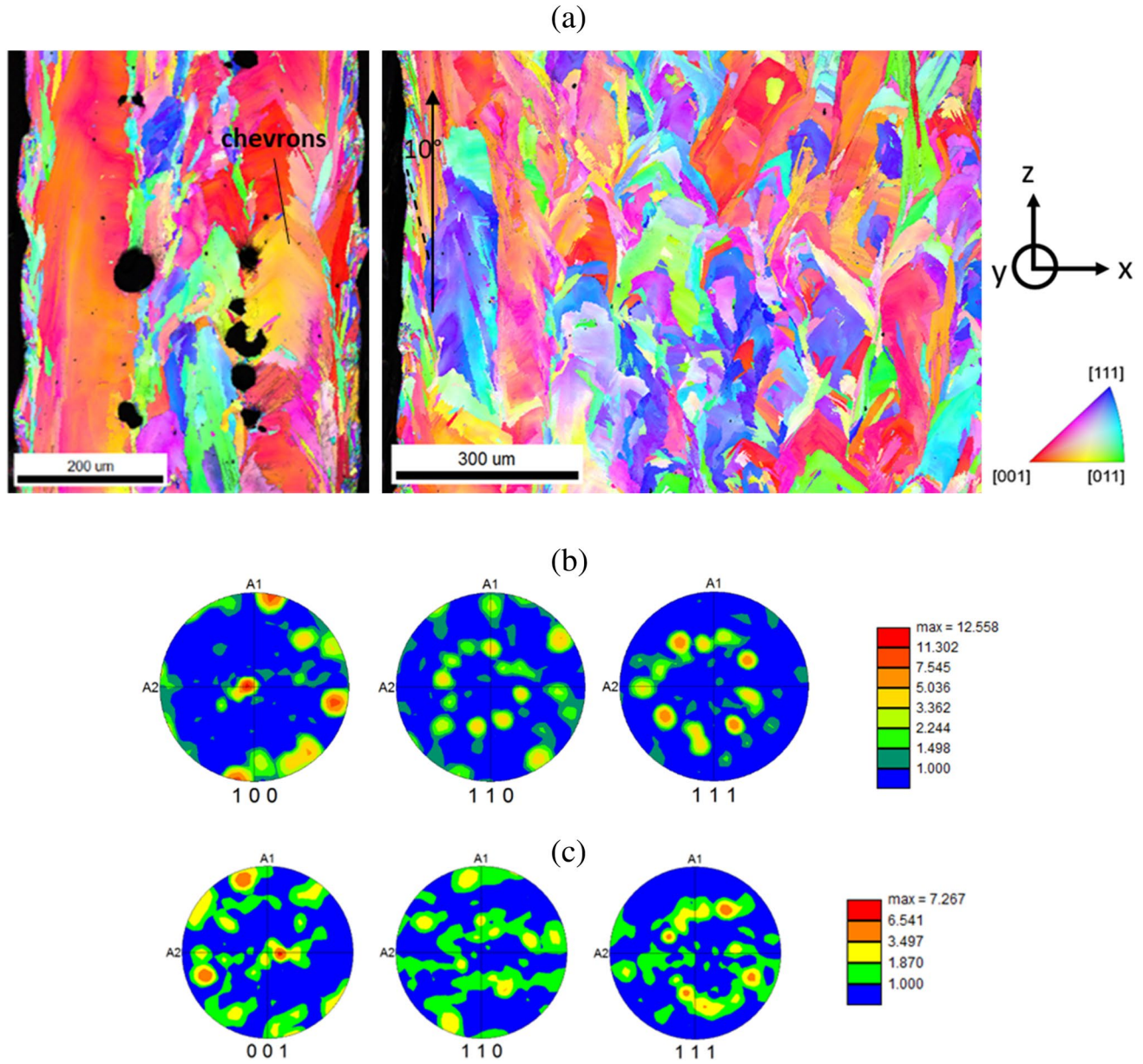
Fig. 25 Longitudinal ( O , x , z ) cross-sectional EBSD-IPF maps: a on a 0.5-mm strut (left) and a 2-mm strut (right) with a CH strategy (IPF map concerning the z -axis), b pole figure (PF) of the 0.3-mm cylinder
