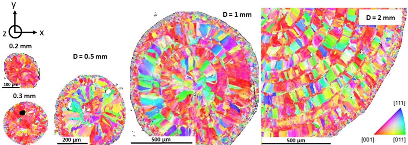
Fig. 24 EBSD analysis of struts. a Transverse ( O, x, y ) cross-sectional EBSD-IPF map concerning the z -axis for (from left to right) for a 0.2-mm strut, a 0.3-mm strut, a 0.5-mm strut, a 1-mm strut, and a 2-mm strut built (IO contouring strategy). b Corresponding pole figures (PF)
