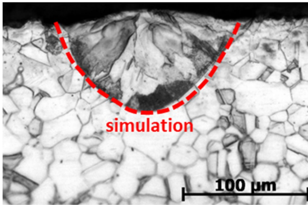
Fig. 8 Calibration of Goldak source parameters on a single L-PBF track (125 W – 0.5 m/s). The best-simulated isotherm is obtained with a_r = a_i = b = 35 \mu\text{m} and c = 70 \mu\text{m}
