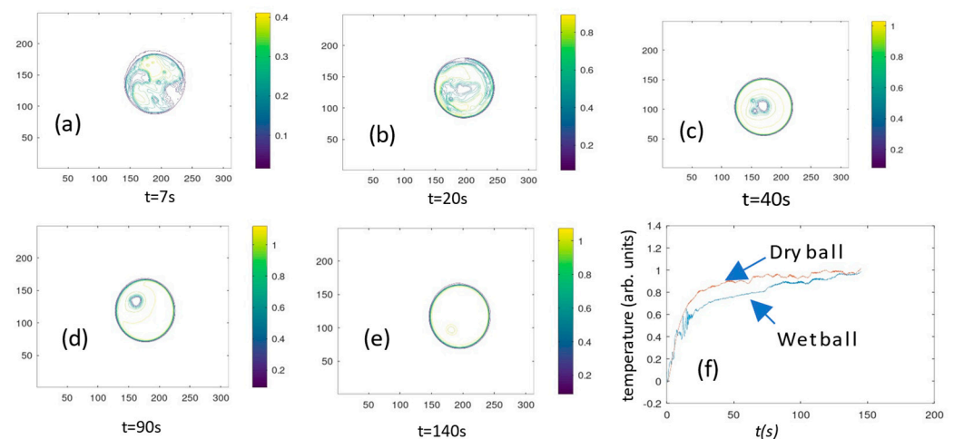
Figure 2. (a–e): Contour-plot of the IR image during convective drying experiment of the ball; (f) averaged temperature evolution comparison between wet and dry ball experiment.
