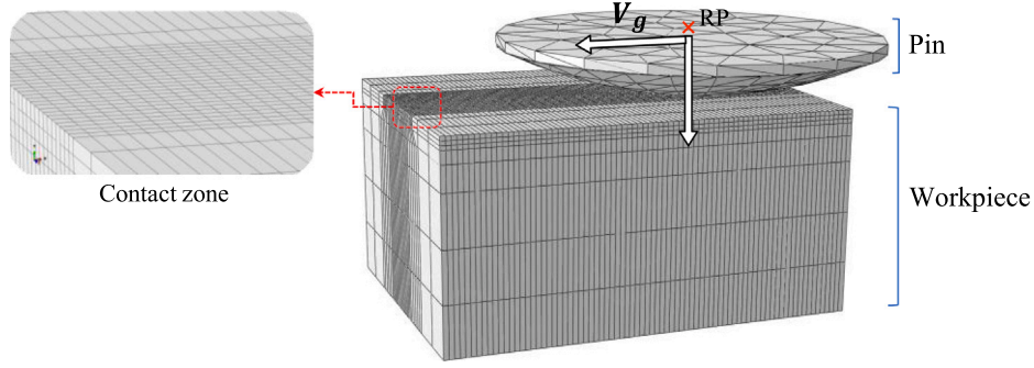
Fig. 3. Geometric model.
