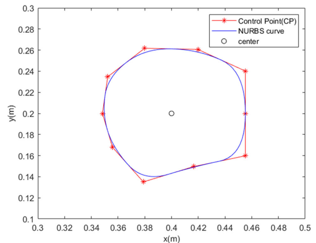
Fig. 4 Illustration of the shape generated by NURBS
