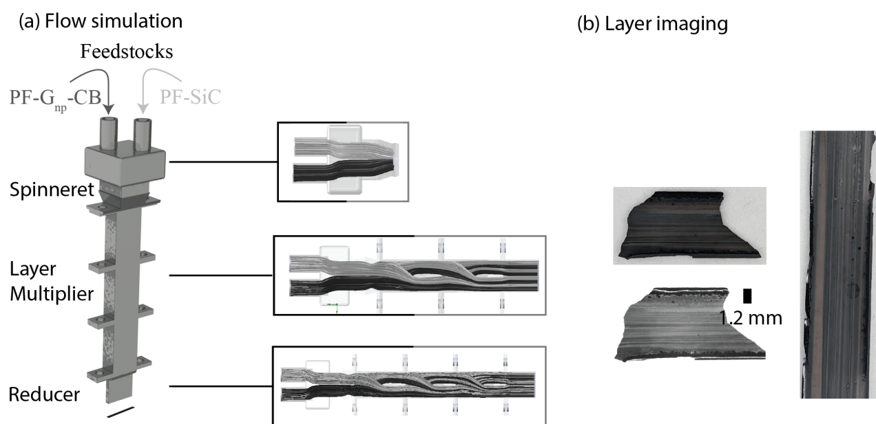
Figure S1: (a) The flow dynamics simulation of double feedstock processing (i.e., PF-SiC and PF-G np -CB as the feedstocks in each printhead channel) with an example of three multipliers in the printhead to produce 16 layers in each printing line and (b) high dynamic range photographs and optical images of as-printed samples showing the distinct layers.
