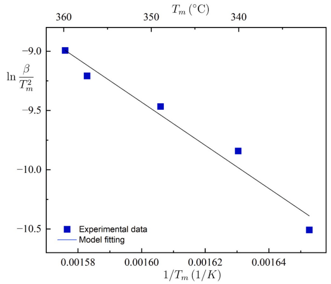
Fig. 4. Kissinger plot of PEFB.
