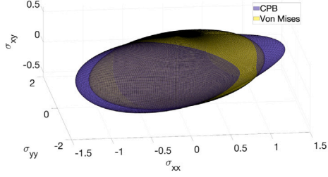
(a) Comparison of yield surfaces.
