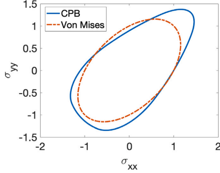
(c) Comparison of yield surfaces at \theta = 90^\circ .
