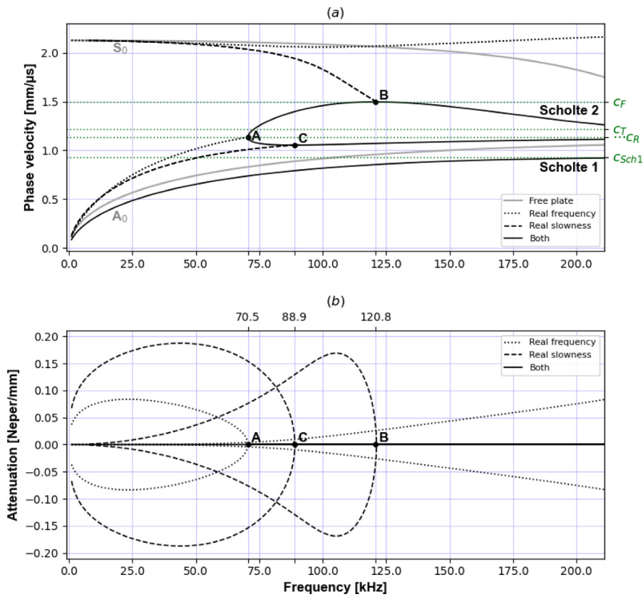
Fig. 2. The phase velocity c_\phi and the attenuation k'' as functions of frequency f = \frac{\omega}{2\pi} , for solutions involving: both real slowness and frequency (—), real frequency (.....), real slowness (---) and a free plate (—). (a) Phase velocity c_\phi (b) Attenuation k'' .
