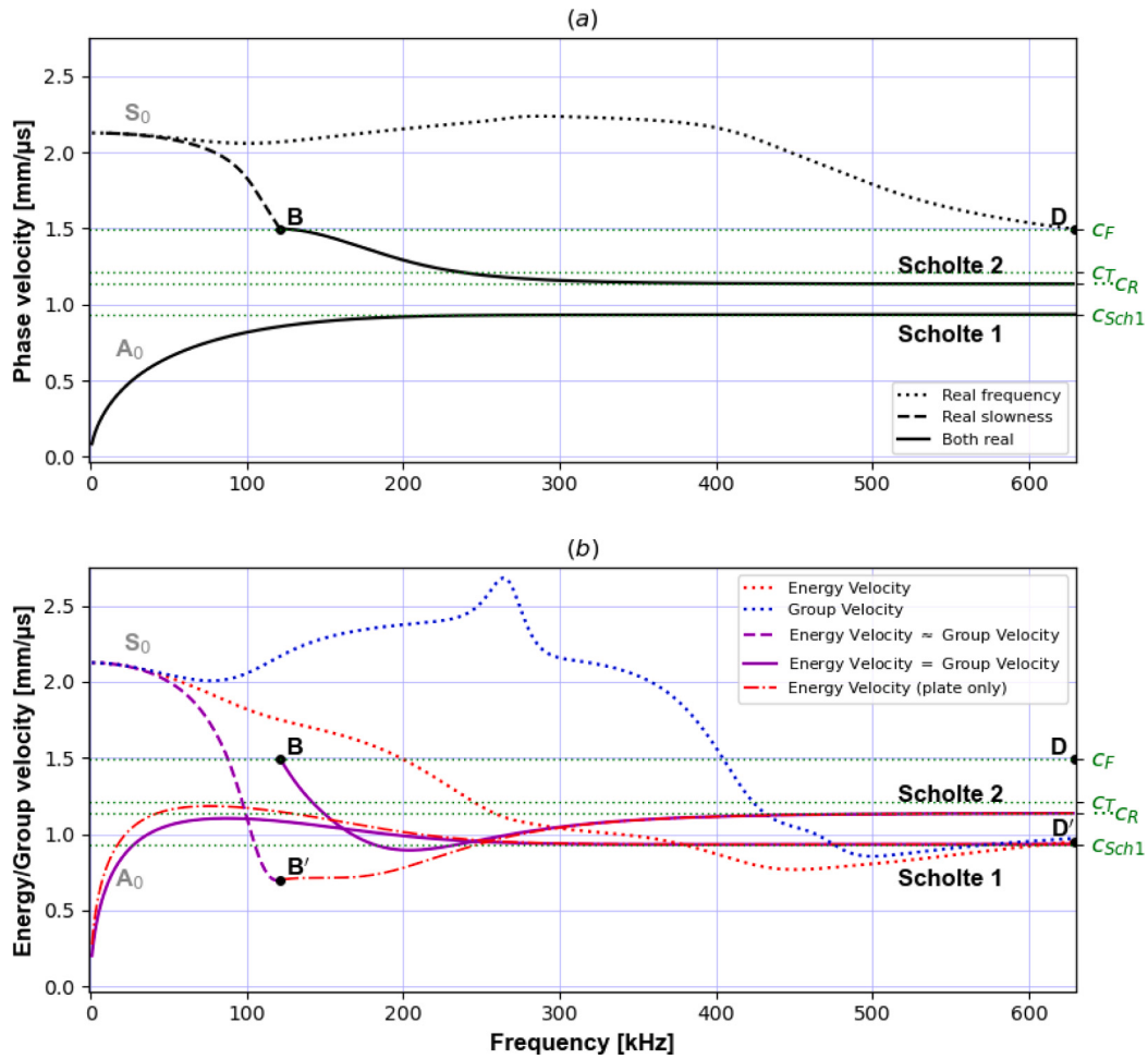
Fig. 3. Group and energy velocities corresponding only to the physical solutions derived from the phase velocity of Fig. 2.a for a frequency range extended. (a) Phase velocity c_\phi for solutions involving: real slowness and frequency (—), real frequency (.....) and real slowness (---). (b) Energy velocity (.....), group velocity (.....), and points where the group velocity equals the energy velocity (—, calculated using Eq. (30)) or approximately equals the energy velocity (---, calculated using Eq. (17)). Energy velocity, for real solutions, calculated using the average from Eq. (17) (---). (For interpretation of the references to color in this figure legend, the reader is referred to the web version of this article.)
