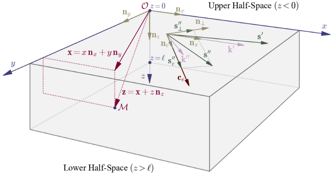
Fig. 1. The plate in the fixed coordinate system (O, \mathbf{n}_x, \mathbf{n}_y, \mathbf{n}_z) , along with the slowness vector \underline{s} and the wavevector \underline{k} associated with the guided wave.
