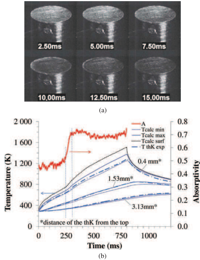
Figure 2 (a) Temporal evolution of the surface of a mild steel rod during laser heating in oxygen during laser irradiation of 1 kW; (b) temporal evolution of a mild steel rod absorptivity during laser irradiation of 180 W, and corresponding measured and calculated temperatures along the rod.
