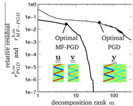
Fig. 4. Comparison of multi-field approach (computed with MF-PGD) and state vector approach (computed with PGD) for TGD P1-P1 scheme. Decompositions are computed with optimal algorithms. Solutions obtained by direct resolution are displayed at the bottom left and right corners.
