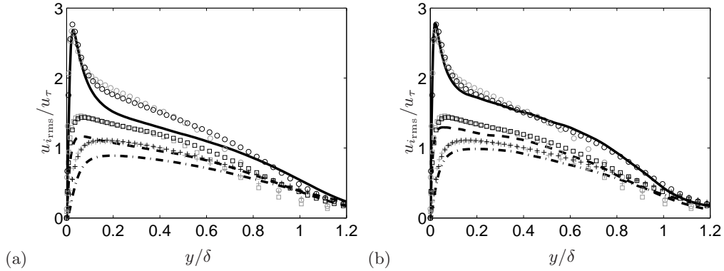
FIGURE 4. Turbulent intensities: u_{1,rms}/u_{\tau} (— present LES; \circ Spalart; \square Jimenez), u_{2,rms}/u_{\tau} ( \cdots present LES; + Spalart; + Jimenez), u_{3,rms}/u_{\tau} ( - - - present LES; \square Spalart; \square Jimenez). (a) coarse-grid LES results at x_1/\delta_{ref}=79.1 , and (b) fine-grid LES results at x_1/\delta_{ref}=73 .
