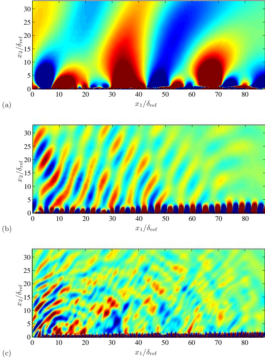
FIGURE 9. Band-pass filtered pressure in the median plane at tU_\infty/\delta_{ref}^*=380.7 : (a) around \omega\delta_{ref}^*/U_\infty=0.033 (range \pm 0.5 Pa), (b) around \omega\delta_{ref}^*/U_\infty=0.20 (range \pm 0.25 Pa), and (c) for the frequency band \omega\delta_{ref}^*/U_\infty \in [0.52; 0.99] (range \pm 1 Pa).
