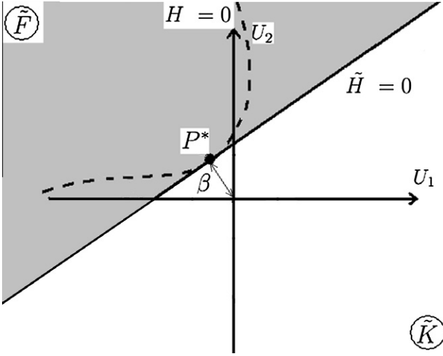
Fig. 7. FORM approach. Representation of approximated regions \tilde{F} and \tilde{K} . \mathbf{U} is the standard space. \beta is the reliability index.
