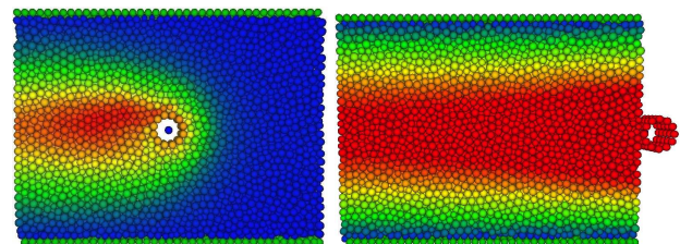
Figure 6: Temperature fields
