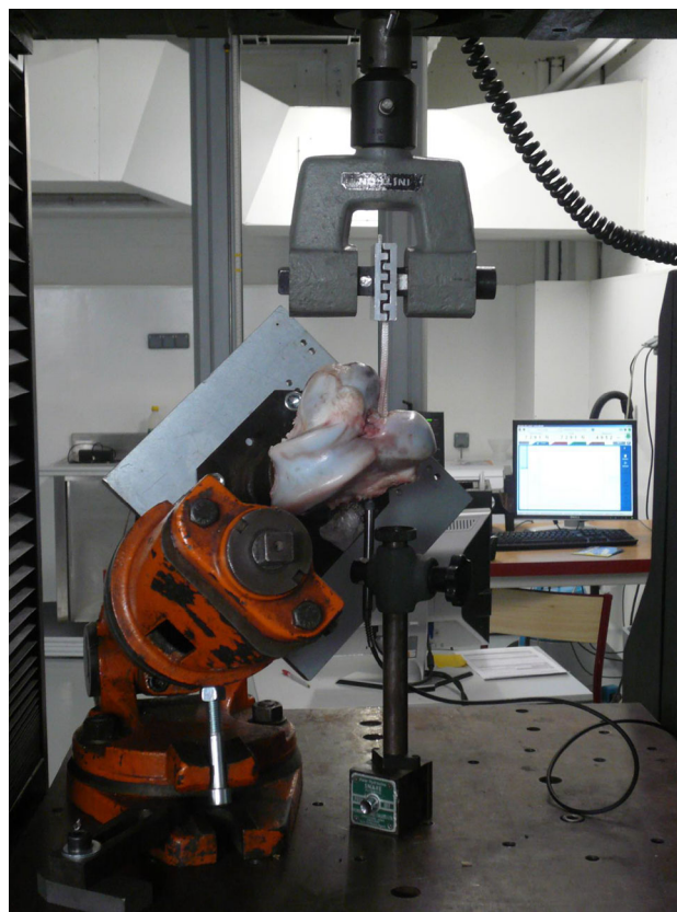
Fig. 3 ACLR loading experimental set-up
