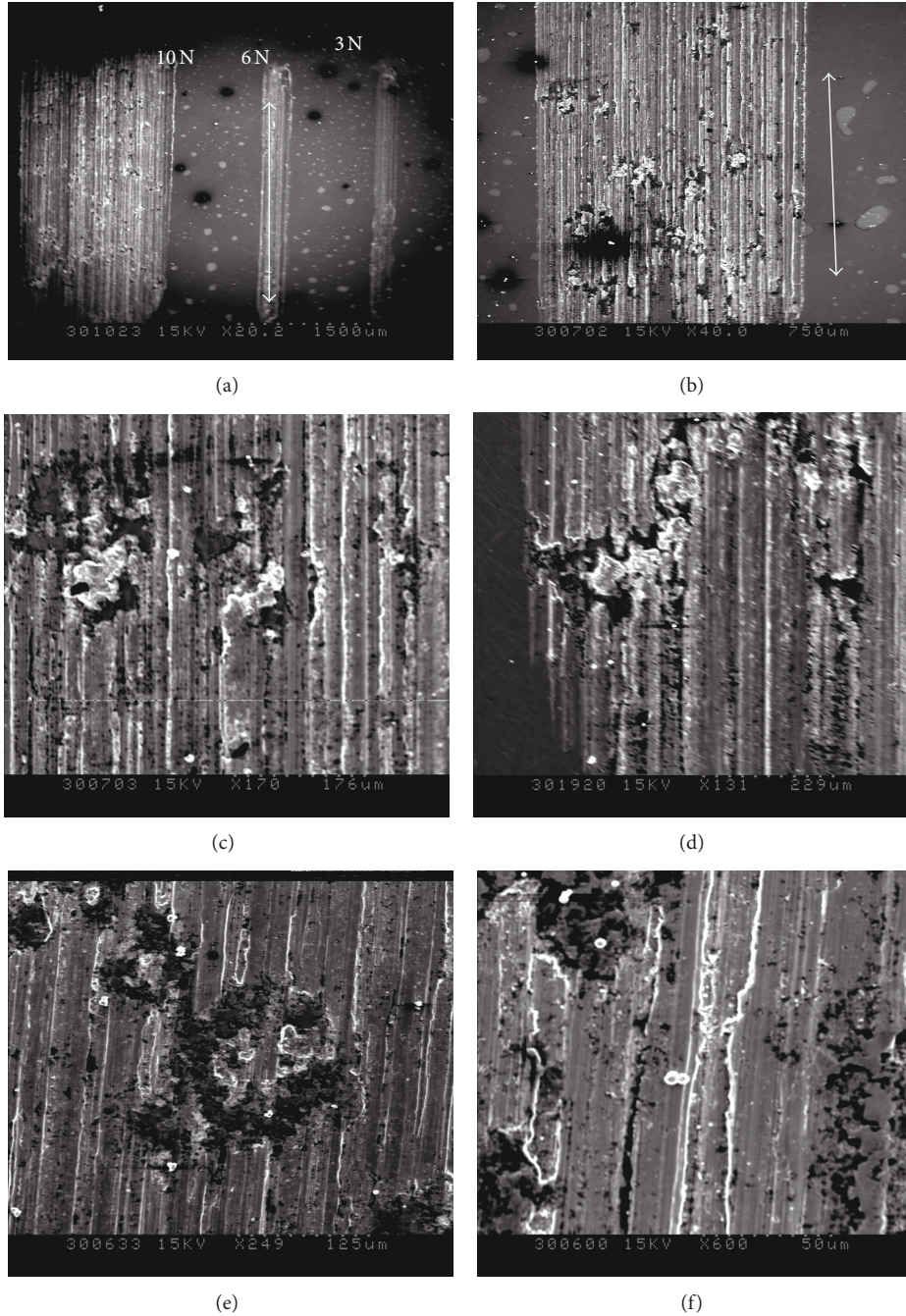
FIGURE 18: SEM micrographs of circular wear marks on Ti-6Al-4V sample after the friction test (severe deformation and plastic flow). Arrows indicate the sliding direction.
