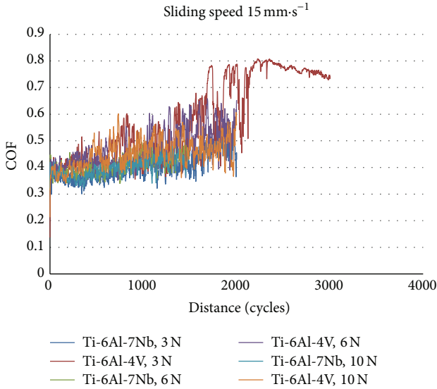
FIGURE 12: Friction coefficient of titanium alloys versus sliding distance at 15 \text{ mm} \cdot \text{s}^{-1} .
