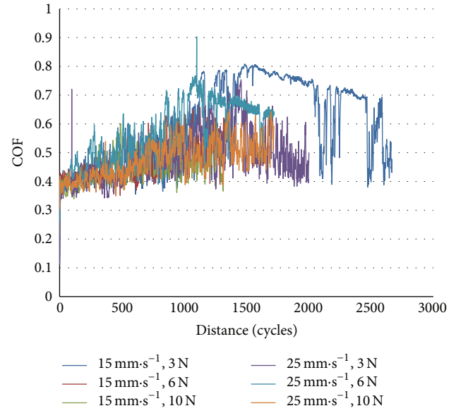
FIGURE 10: Friction coefficient of Ti-6Al-4V alloy versus sliding distance at tow sliding speed (15 and 25 mm·s -1 ).
