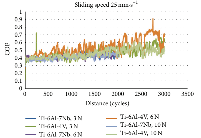
FIGURE 13: Friction coefficient of titanium alloys versus sliding distance under different conditions of loads at 25 \text{ mm} \cdot \text{s}^{-1} .
