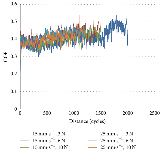
FIGURE 9: Friction coefficient of Ti-6Al-7Nb alloy versus sliding distance at tow sliding speed (15 and 25 mm·s -1 ).
