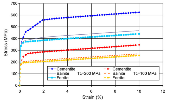
Fig. 7. Influence of the initial value of the critical resolved shear stress (100 and 200MPa) on the stress distribution ( \sigma_{11} component) in a bainitic single crystal (Mori-Tanaka model, f=0.15 ): predicted overall average stress as well as stress averages in ferrite and cementite phases are plotted as a function of the overall strain ( \varepsilon_{11} component).
