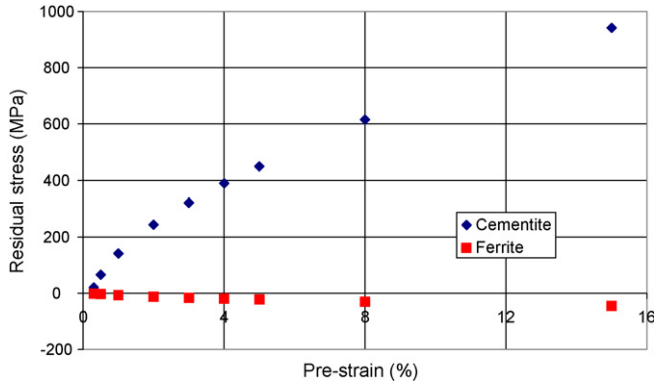
Fig. 13. Evolution of the simulated residual average stress ( \sigma_{11}^r component after complete unloading) in ferrite and cementite as a function of the macroscopic tensile strain in the 16MND5 steel ( -60^{\circ}\text{C} ).
