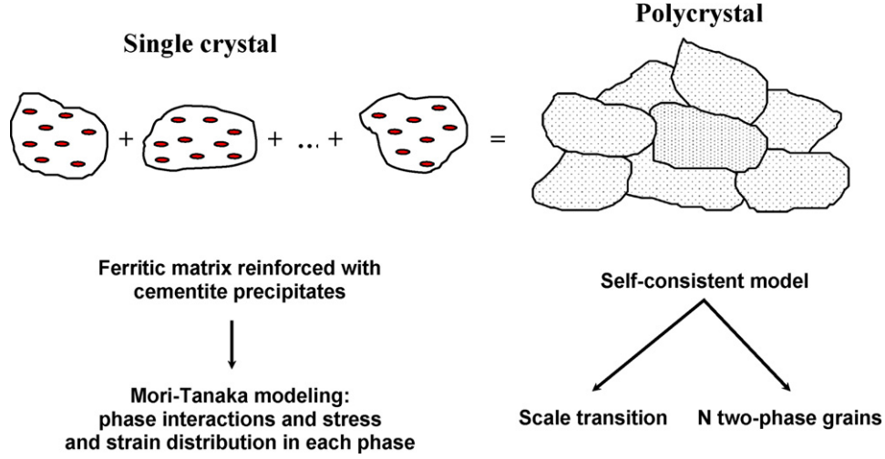
Fig. 1. Polycrystalline modeling with a two-level homogenisation.
