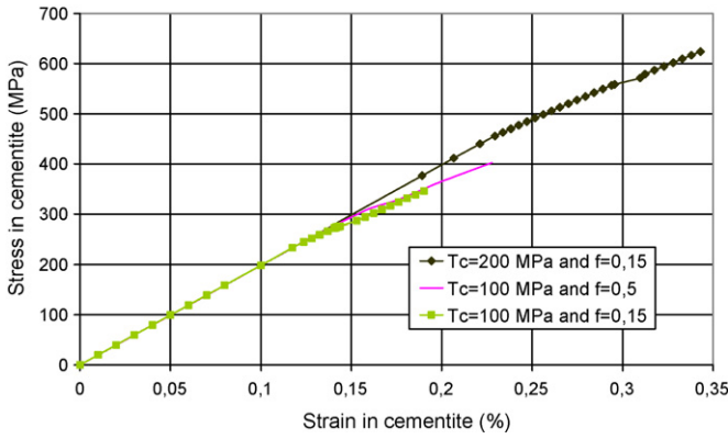
Fig. 5. Average stress ( \sigma_{11} component) in cementite (Mori-Tanaka model: bainitic single crystal) as a function of the average strain in cementite ( \varepsilon_{11} component): influence of the initial value of the critical resolved shear stress ( T_c ) and the volume fraction of cementite ( f ).
