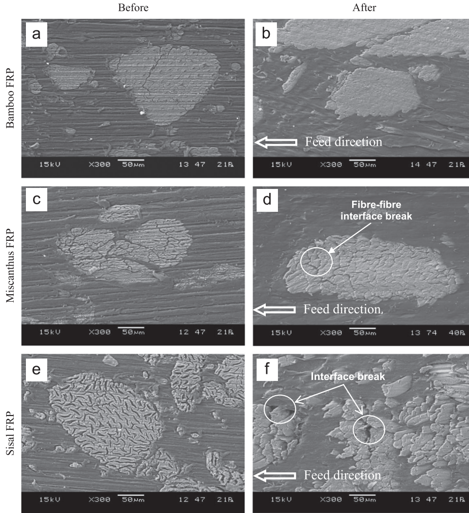
Fig. 3. SEM image of surface state of NFRP before and after profile milling process at f_2=0.04 mm/tooth.
