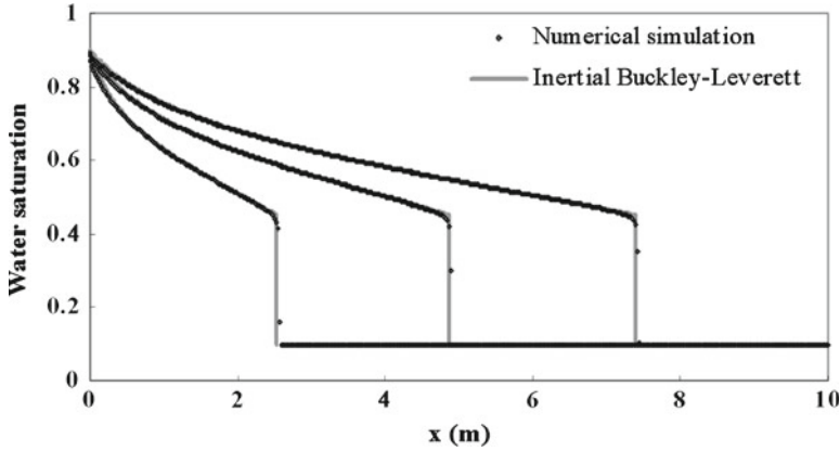
Fig. 1 Comparison of saturation profiles for various times ( t = 10.4\text{ s} , 20\text{ s} , and 30.4\text{ s} ) obtained by the numerical code with those resulting from the semi-analytical resolution of the Buckley–Leverett type; number of grid-blocks N = 400 , \Delta t = 0.08\text{ s}
