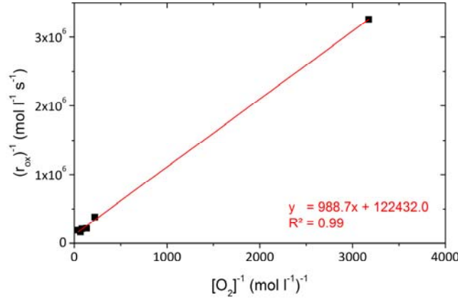
Figure 9. 1/r_{ox} vs 1/[O_2] plot at 110 °C.
