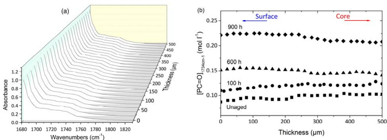
Figure 3. IR spectra in carbonyl area across a sample aged 900 h under air at 110\text{ }^{\circ}\text{C} (a) and the carbonyl build as a function of aging time across the section of aged samples under air at 110\text{ }^{\circ}\text{C} (b).
