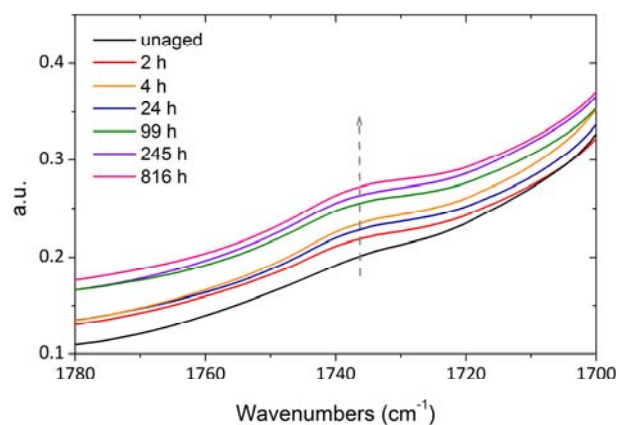
Figure 12. IR spectra (carbonyl area) for PA11 film samples aged under N_2 (0.5 MPa) at 150 °C.
