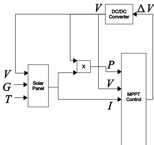
Fig. 3. The principle of MPPT control
