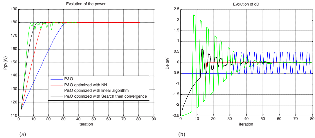
Fig. 8. Four MPPT control algorithms (a) Evolution of P_{pv} . (b) Evolution of \Delta V
