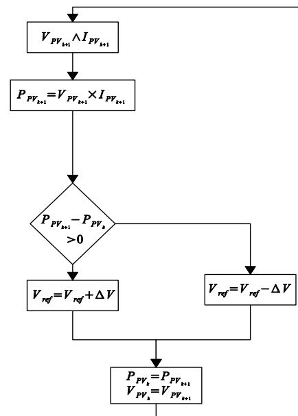
Fig. 4. The principle of P&amp;O MPPT control
