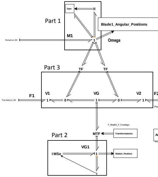
Figure 10. MBG of a moving rigid body - Example of a blade
