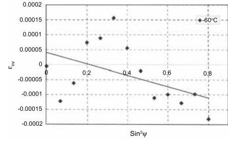
Fig.5 \varepsilon_{\phi\psi} = f(\sin^2\psi) strains calculated with the model after unloading (tensile test, 8% strain rate)
