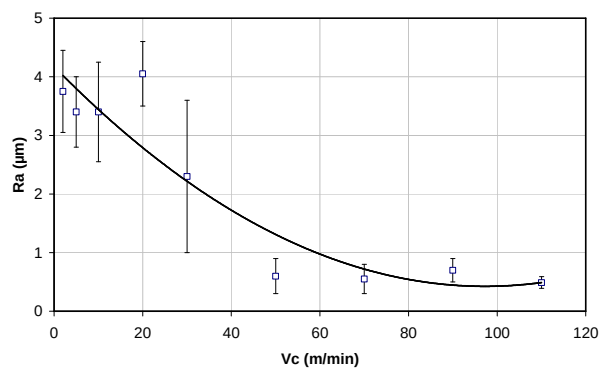
Figure 12 : Roughness measurement N - f = 0,2 mm/rev - dry
