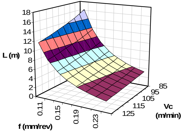
Figure 20 : Drilled length versus V_c and f G - dry
