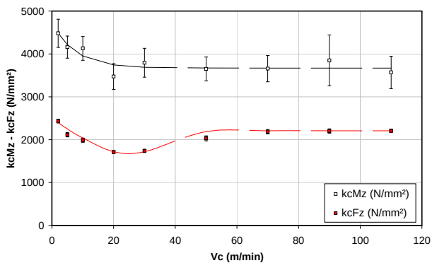
Figure 10 : V_{c_{min}} from kc_{Mz} and kc_{Fz} computations N - f = 0,15 mm/rev - dry
