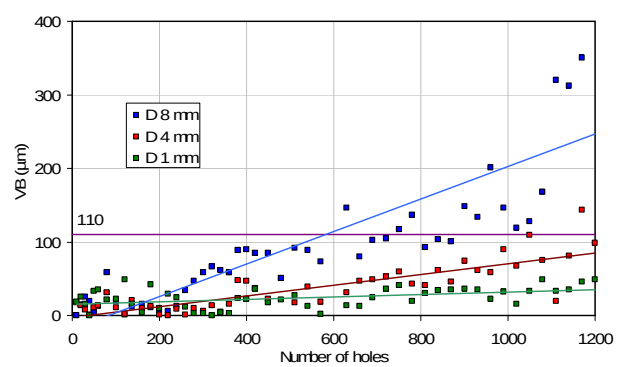
Figure 18 : Tool wear evolution G - V_c = 85 \text{ m/min} - f = 0.11 \text{ mm/rev} - dry
