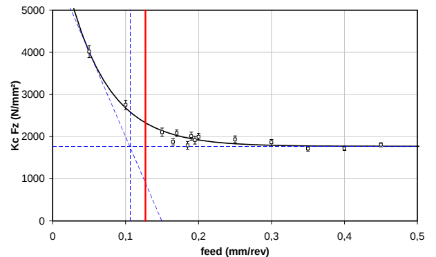
Figure 5 : f_{min} from K_{C_{F_z}} computations G - V_c = 85 m/min - dry
