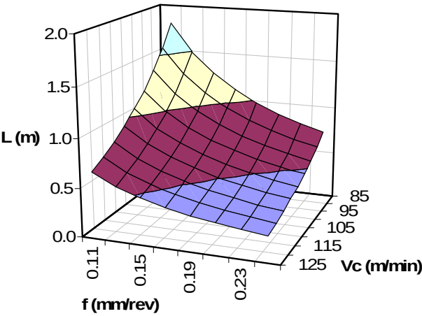
Figure 19 : Drilled length versus V_c and f N - dry
