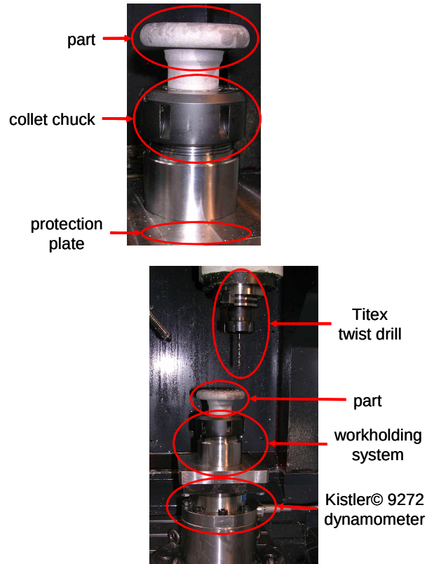
Figure 2 : Work holding device for force measurement tests
